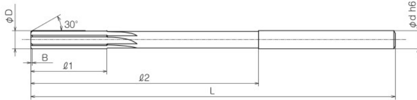
(φ2.910mm~φ18.030mm形状) (φ2.910mm - φ18.030mm Dia. shape)
