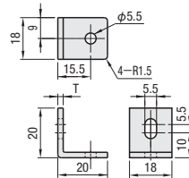
HPTBS5 SHPTBS5
