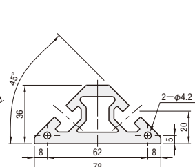
NFSR8-4040 HFSR8-4040
