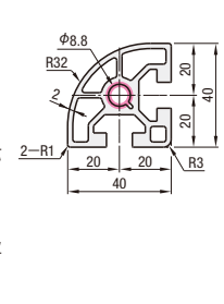
NFSR8-4040 HFSR8-4040
