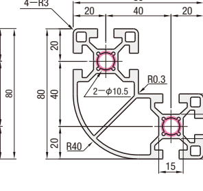
NFSR8-808040 HFSR8-808040
