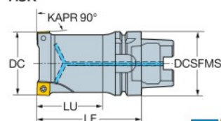
HSK
